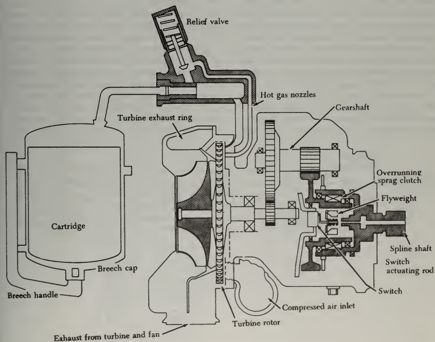
FIGURE 5-21. Cartridge/pneumatic starter schematic.
